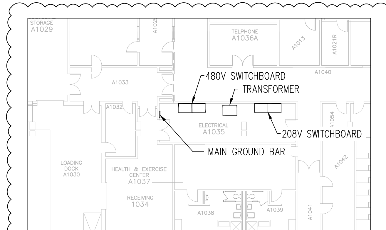
ENLARGED FLOOR PLAN
