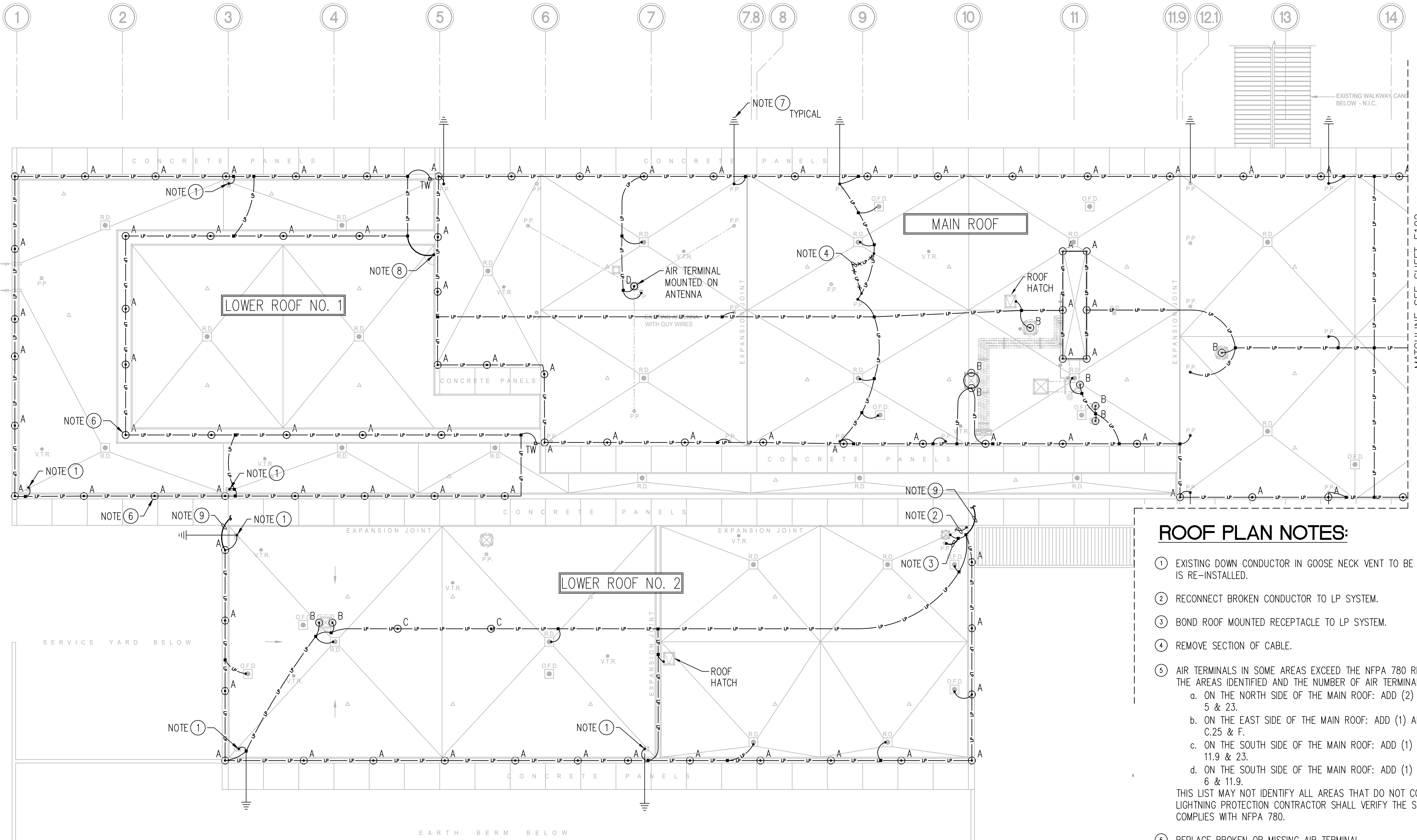
PARTIAL ROOF PLAN LIGHTNING PROTECTION SCALE: 1/16" = 1'-0"
